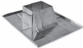
Flashing with 4 sides for tiles or bent tiles
